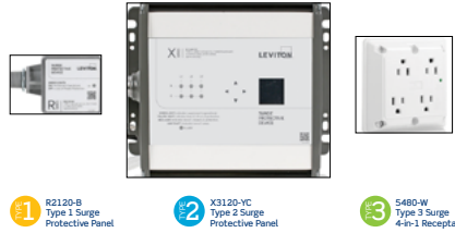
Surge Protective Devices
