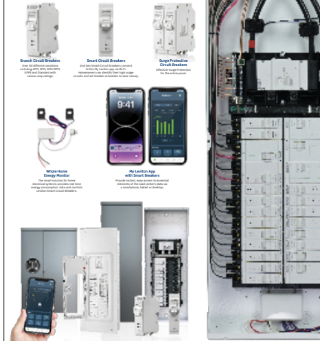
The Leviton Load Center
