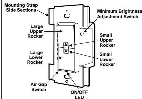
Figure 1 - Dimmer Functions
