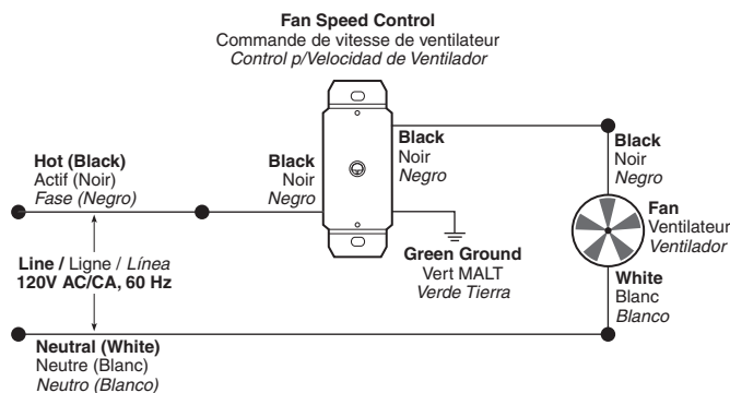
Wiring Diagram - Single Location Control Application
