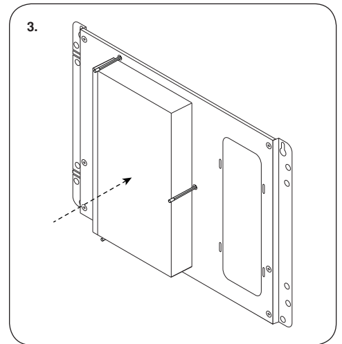
3. Place the POENS-8PT PoE switch onto the POEMP-KIT so that the rubber feet attached in step 1 make contact with the POEMP-KIT as shown (The POENS-8PT product ID Label should be facing you).
