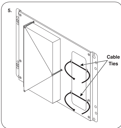
5. Install cable ties on POEMP-KIT as shown.
