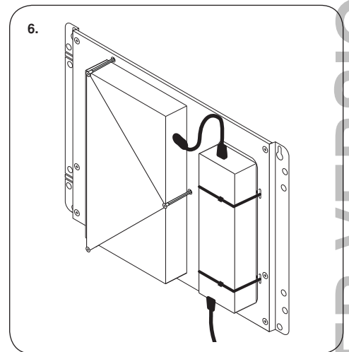
6. Plug power supply into the POENS-8PT PoE switch and secure power supply to the POEMP-KIT as shown.
