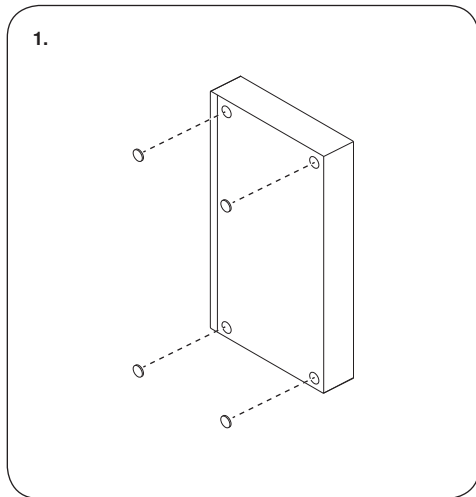
1. Attach the 4 rubber feet provided with the POEMP-KIT onto the top of the enclosure of the POENS-8PT 8 Port PoE switch as shown.
