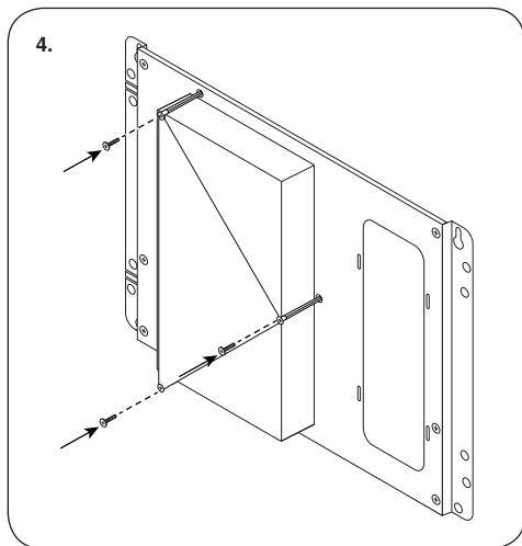
4. Attach triangular retention plate using provided screws.
