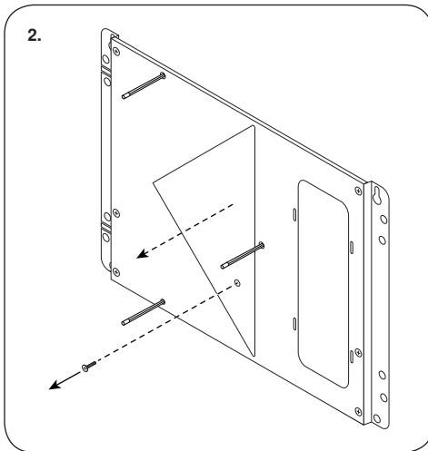
2. Remove the screw that holds in the triangular retention plate ( save this screw for step 4 ).
