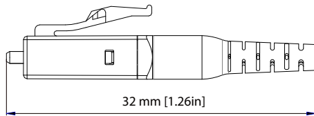
Simplex with boot for 900µm fiber
