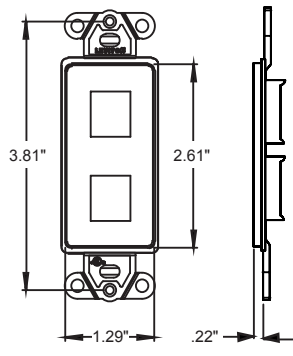
2-Port Insert
