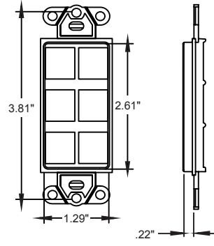
6-Port Insert
