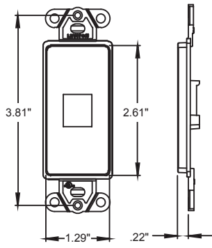
1-Port Insert
