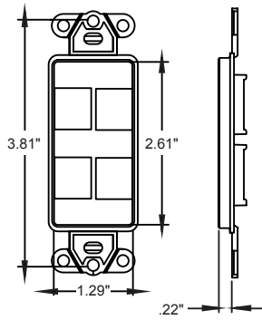
4-Port Insert
