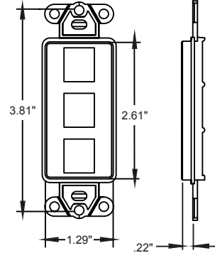
3-Port Insert
