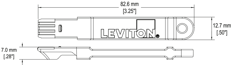
EXTRACTION TOOL
