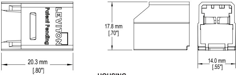
HOUSING
