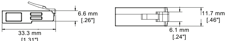
PLUG
