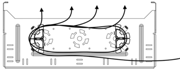
ROUTE FIBER CABLING EVENLY FROM ONE DIRECTION OF A RACK OR CABINET UTILIZING WIRE MANAGEMENT RINGS FOR BEST RESULTS
