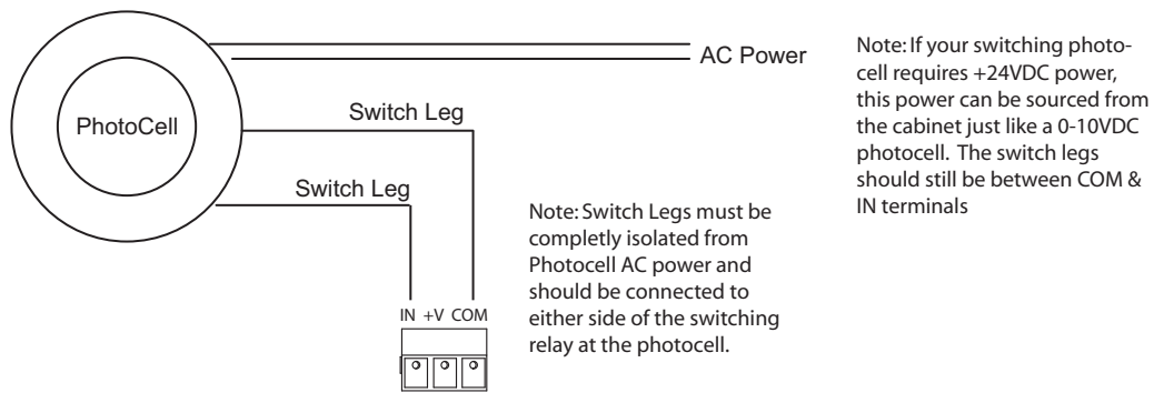
Figure 7-2: Switching Photocell
