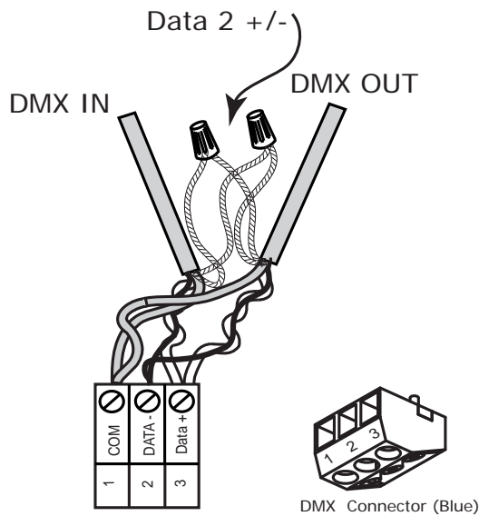
Figure 11-1: Z-Max DMX connector wiring
