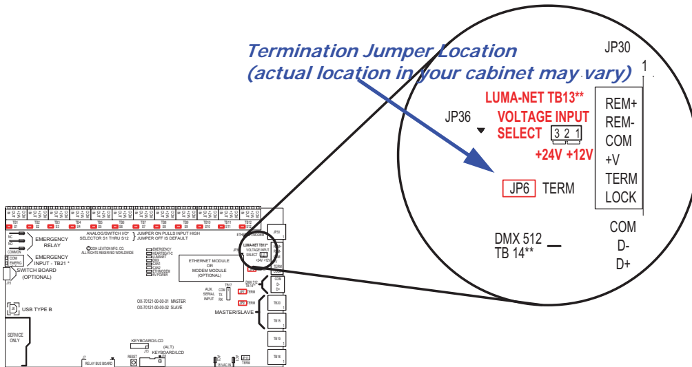
Figure 10-1: Typical termination jumper location
