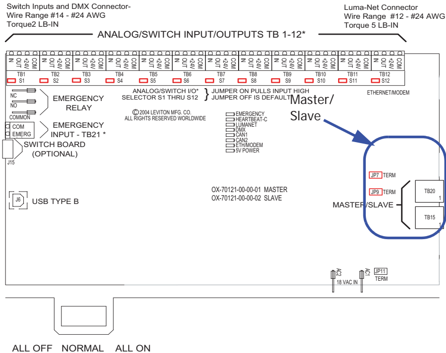
Figure 9-3: Master/Slave Connections Z-MAX 24, & 48 Relay Panel
