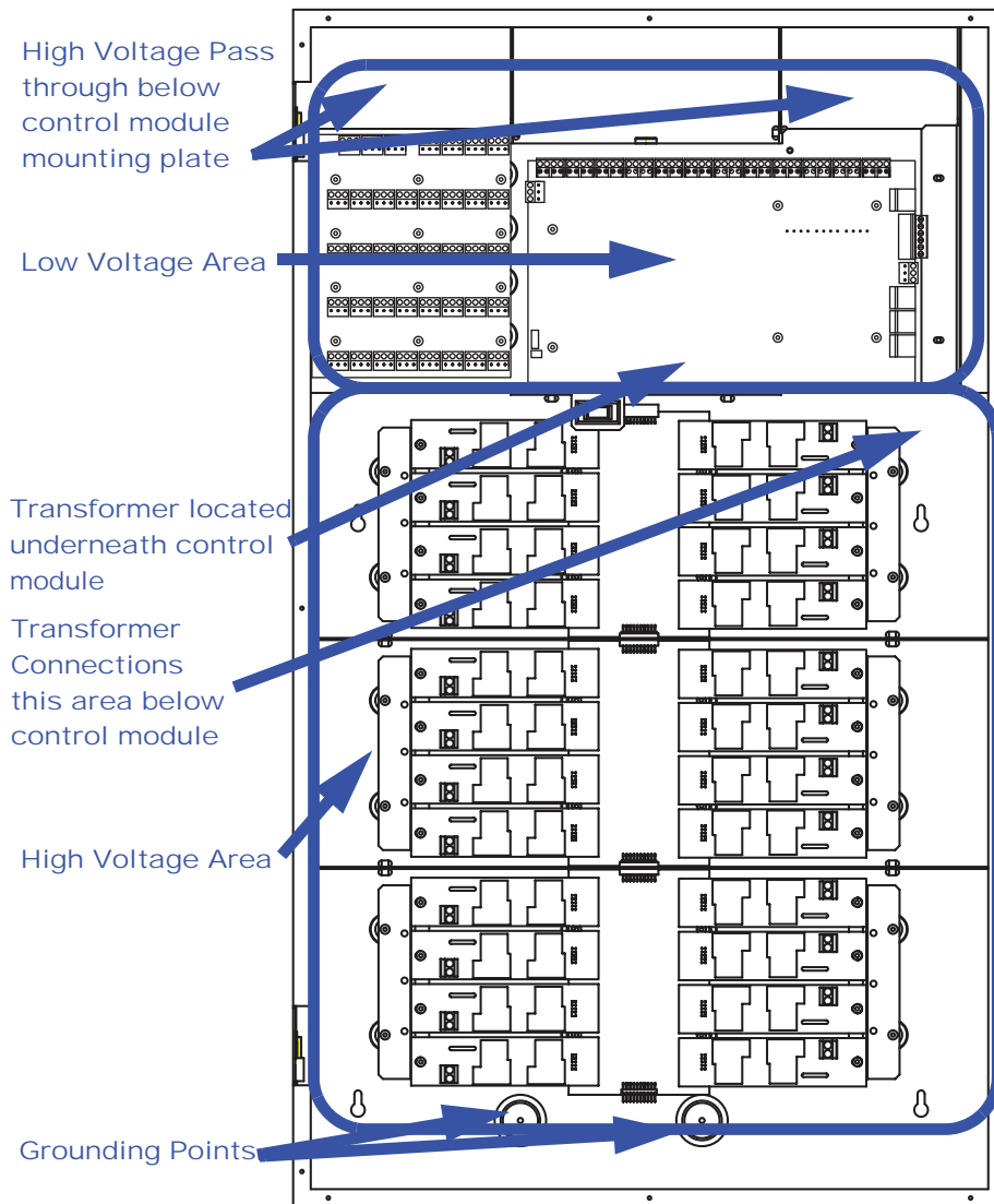
Figure 3-1: 24 Cabinet Low Voltage and High Voltage Wire Connections (48 similar)
