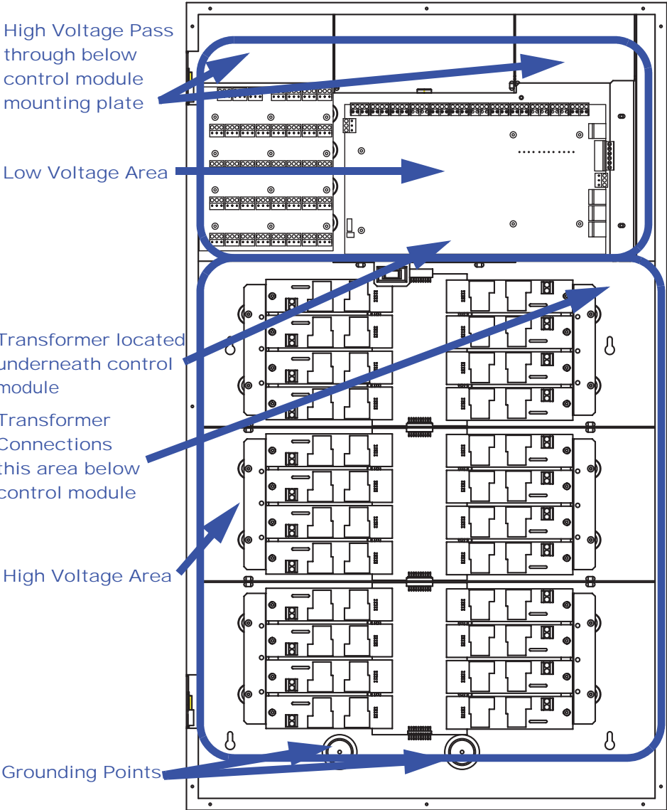
Figure 2-2: 24 & 48 Relay Cabinets Conduit Entry (24 relay cabinet shown, 48 similar)
