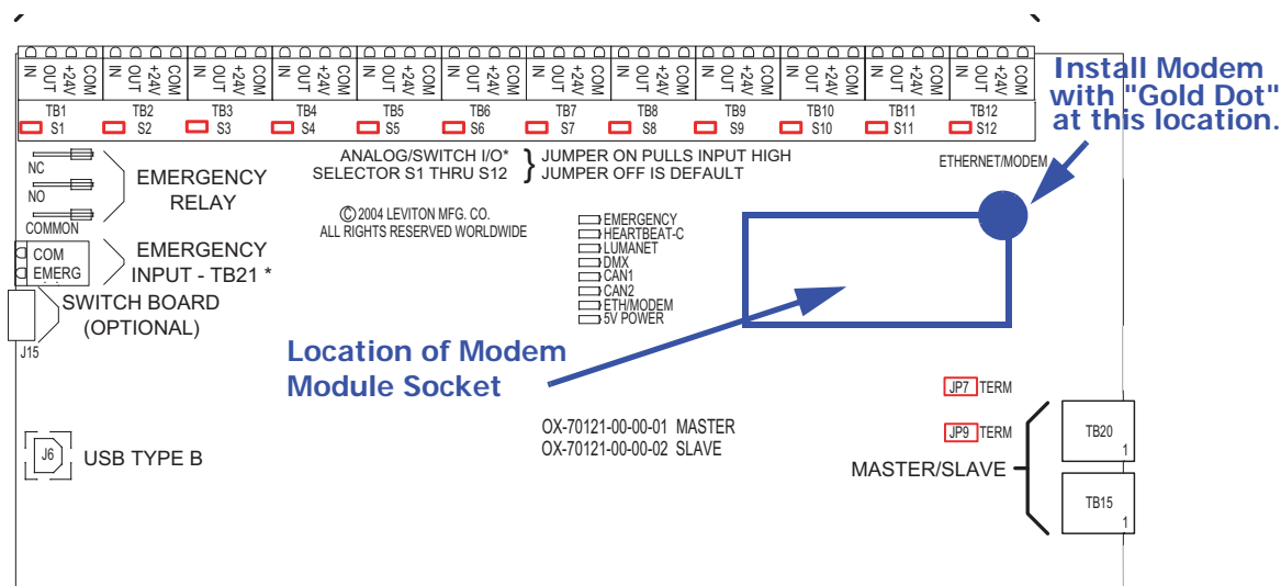
Figure 12-1: Modem Module Installation, 24 & 48 relay cabinets
