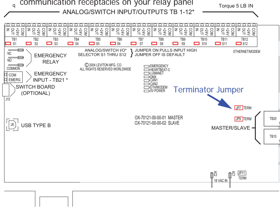
Figure 9-1: 24/48 relay panel control module shown, others similar
