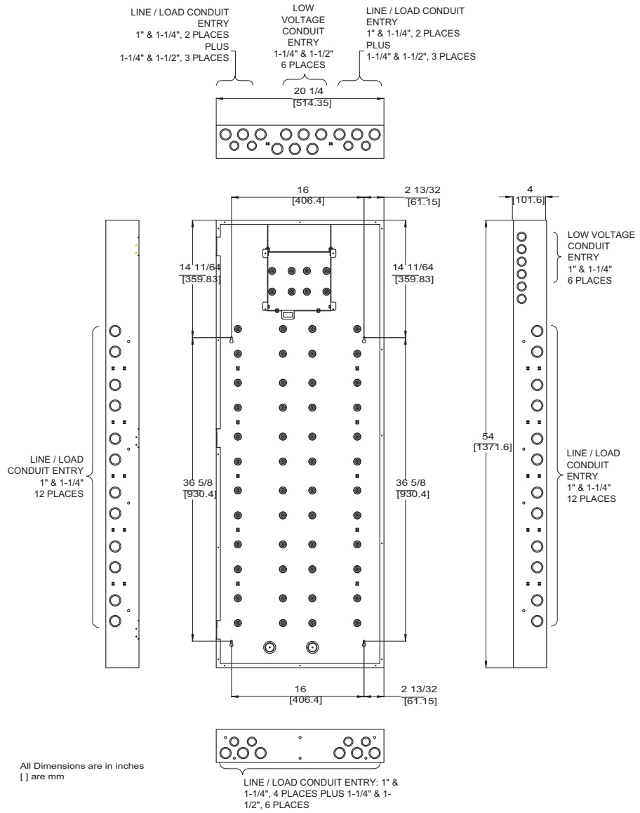
Figure 2-5: Z-Max 48 Relay cabinet mounting provisions and dimensions
