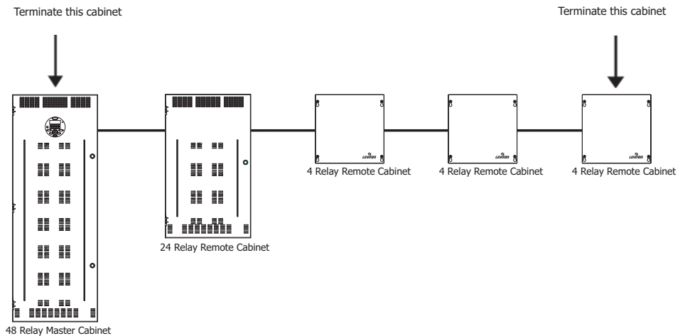
Figure 9-4: Cabinets requiring termination
