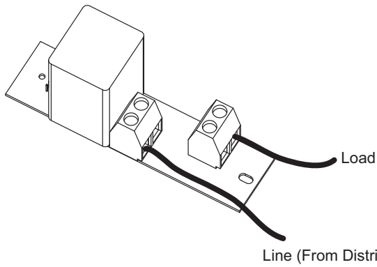
Figure 3-3: Wiring Diagram for Z-Max 347 V Relay Card
