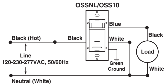
OSS10 Wall Switch Occupancy Sensor Wiring Diagram, Single Location Control
