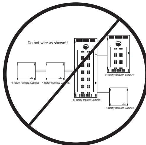
The wrong way - Star or other scheme
