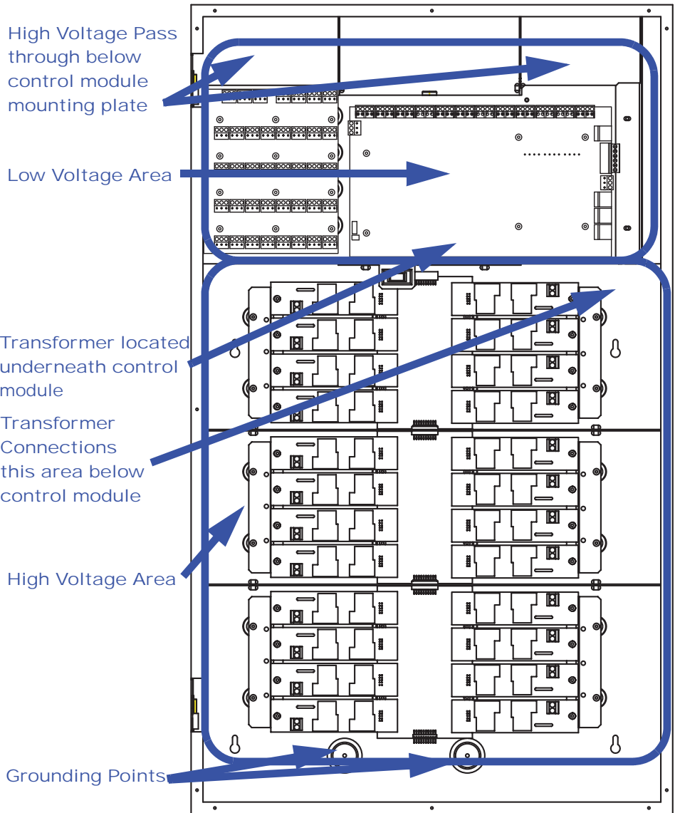
24 & 48 Relay Cabinets Conduit Entry (24 relay cabinet shown, 48 similar)
