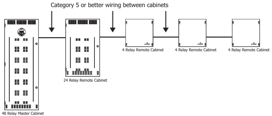
The right way - Daisy-Chain Wiring
