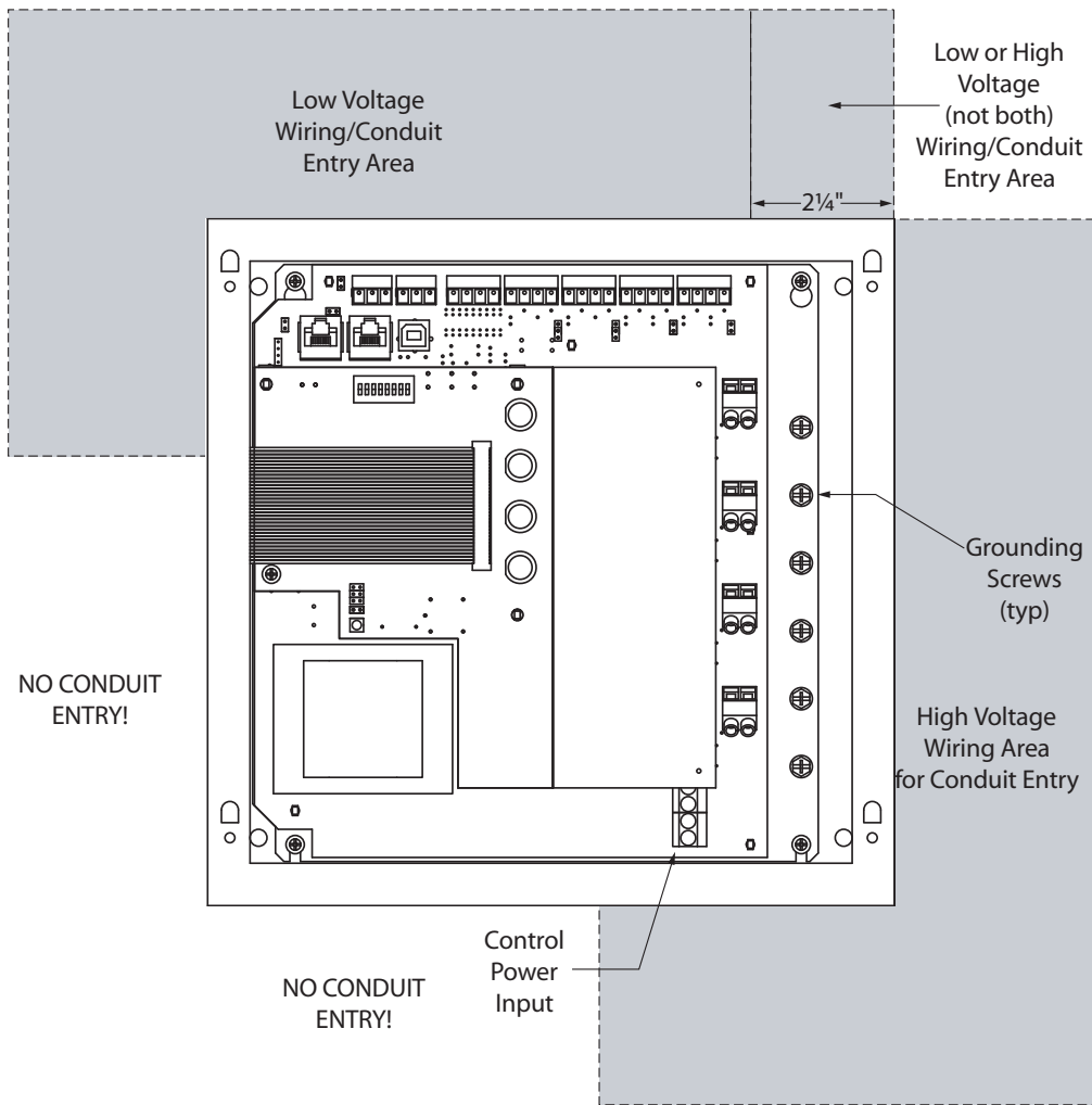
4 Relay Cabinet Conduit Entry
