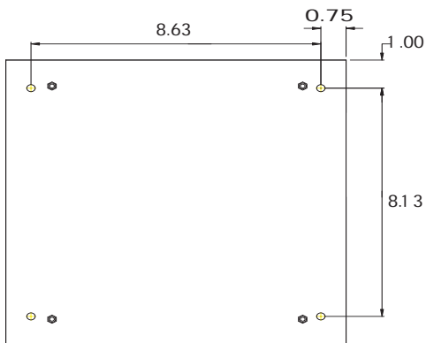
MOUNTING HOLES VIEW (all dimensions in inches)
