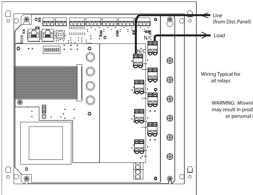
Wiring Diagram for 4 Relay Panel 347V Canadian Relay
