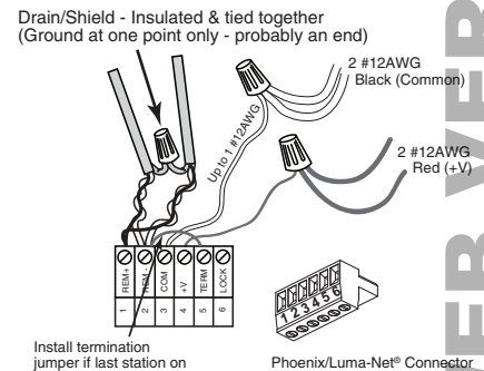
Luma-Net® Wire Connections for runs longer than 1,000 ft.
