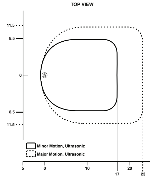
Figure 2 (Cat. No. OSC05) Field-of-View Ranges
