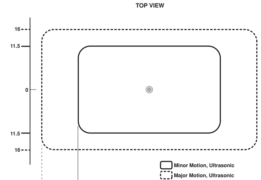
Figure 4 (Cat. NO. OSC20) Field-of-View Ranges
