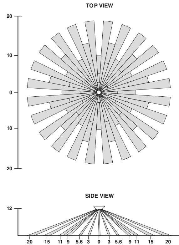
Figure 6 - (Cat. No. O2C15) Field-of-View Ranges Extended range lens (black frame), mounting height (8-12 ft)
