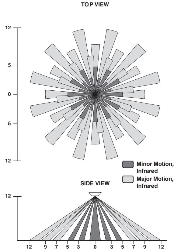
Figure 6 - (Cat. No. O2C15) Field-of-View Ranges Extended range lens (black frame), mounting height (8-12 ft)
