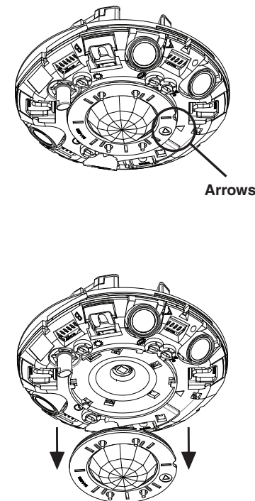
Figure 8 - Changing PIR Lens To change lens, turn lens and line up arrows, then pull lens from sensor
