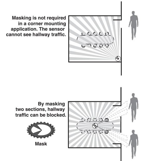
Figure 9 - Mounting Location Diagram
