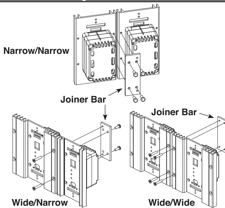
Figure 5 - Joiner Bar
