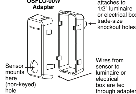
OSFOA-00W Adapter
