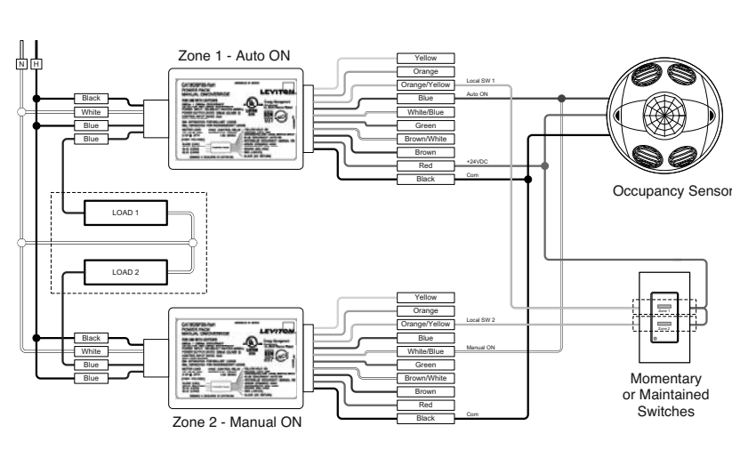
OSP20-RxH Bi-Level Switching
