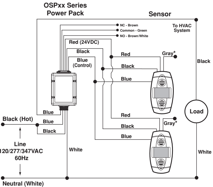
Wiring Diagram Multiple Sensor, Single Power Pack
