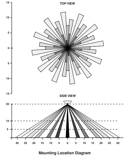
Figure 5 - (Mid-Range Lens) Field-of-View Ranges Note: This lens is included with all PIR models.
