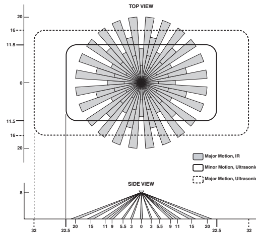
Figure 4 (Cat. No. OSC20) Field-of-View Ranges
