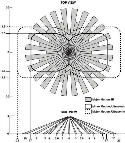
Figure 3 (Cat. No. OSC10) Field-of-View Ranges
