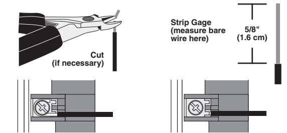
Side Wire Connection Side wire terminals accept #14-12 AWG solid copper wire only.
