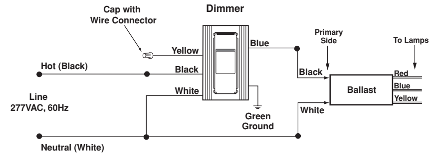
Wiring Diagram 2 – Two Location Control Application
