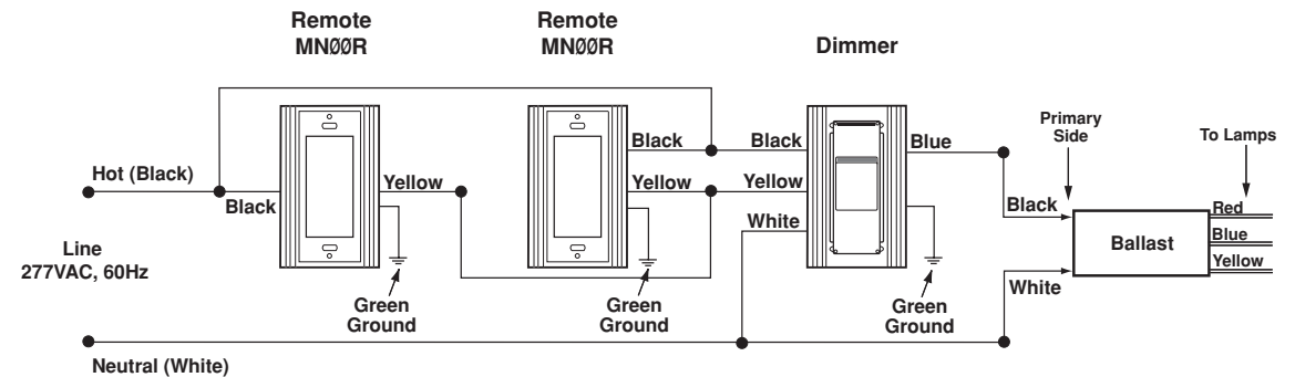
Wiring Diagram 3 – Three Location Control Application
