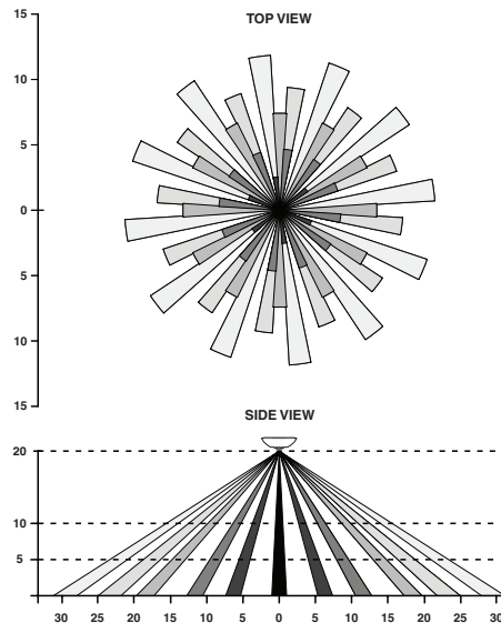
Figure 4 - (Mid-Range Lens) Field-of-View Ranges
