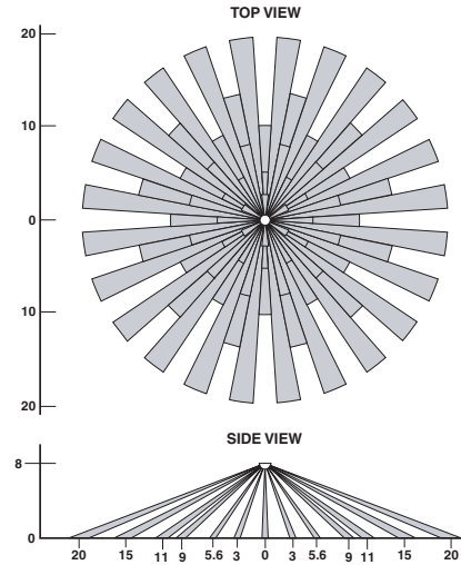
Figure 4 - (Mid-Range Lens) Field-of-View Ranges
