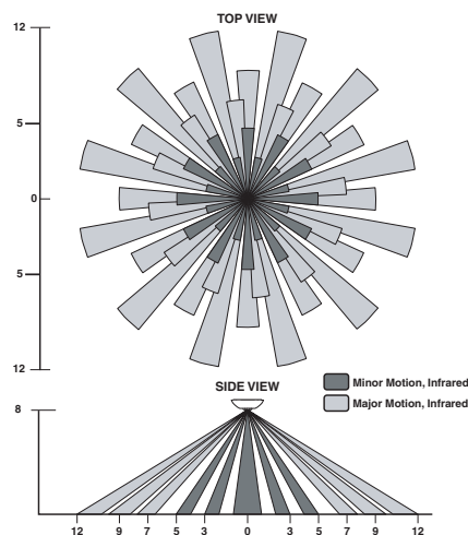
Figure 2 - (Cat. No. OSC04) Field-of-View Ranges
