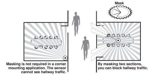
Mounting Location Diagram
