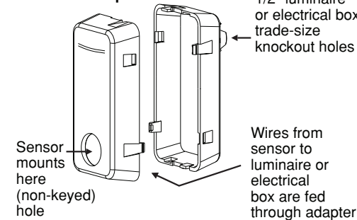
OSFLO-00W Adapter
