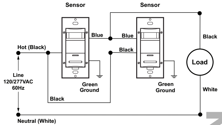
Wiring Diagram 2 - Two Location Control Application
