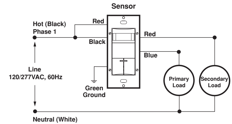
Wiring Diagram 1 - Single Control Application
