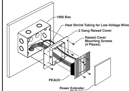
Figure 1A: Surface Mounting
