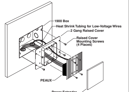
Figure 1B: Flush Mounting
