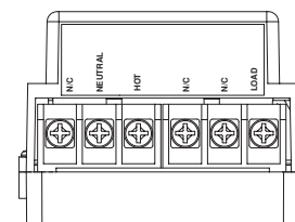
Figure 2: End View
