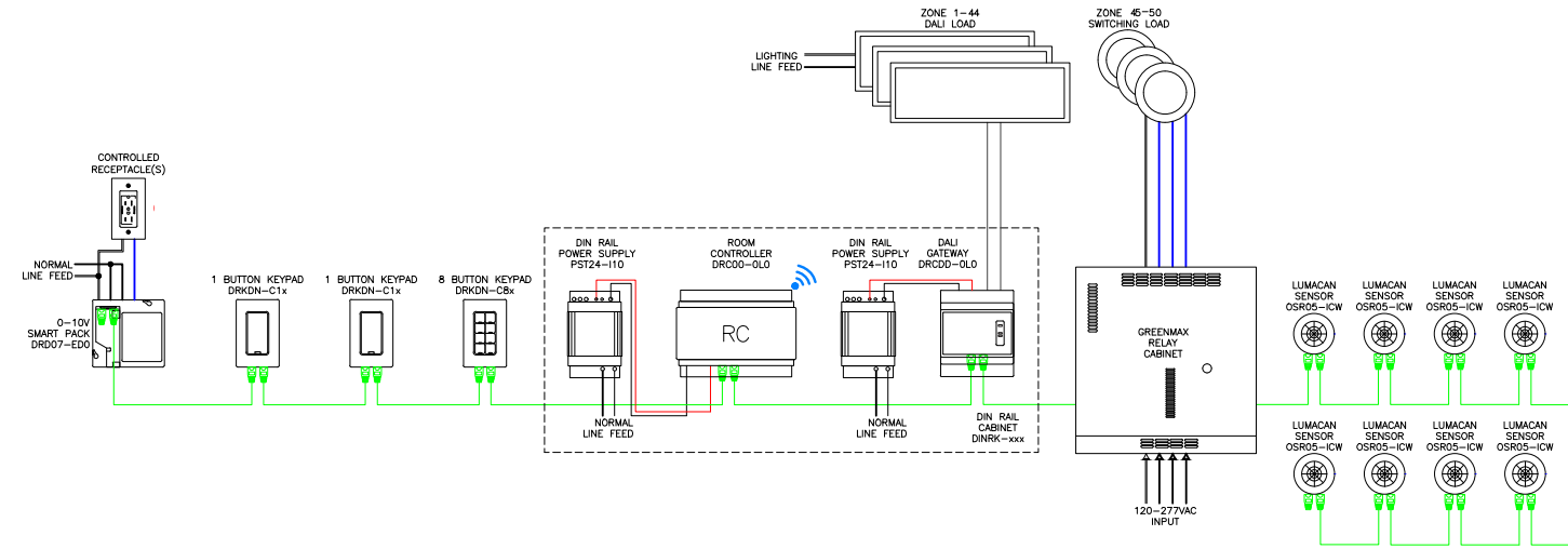
GreenMAX DRC 70-Zone DALI and 8-Zone Relay Plus Daylighting, Typical
