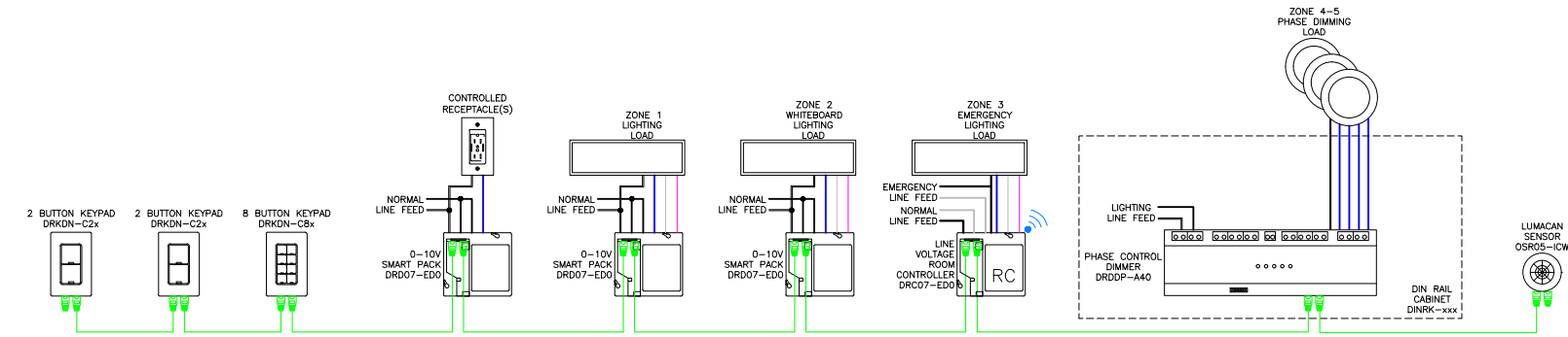
GreenMAX DRC 3-Zone 0-10V and 2-Zone Phase Control Dimming Plus Daylighting, Typical
