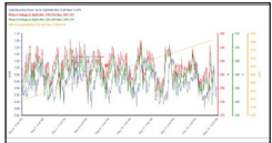
BMO 2.0 Software
