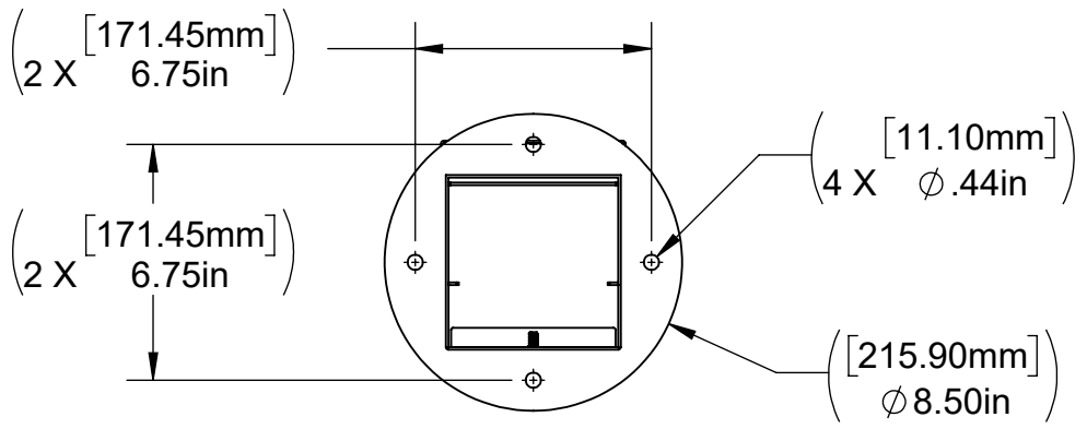
MOUNTING HOLES
