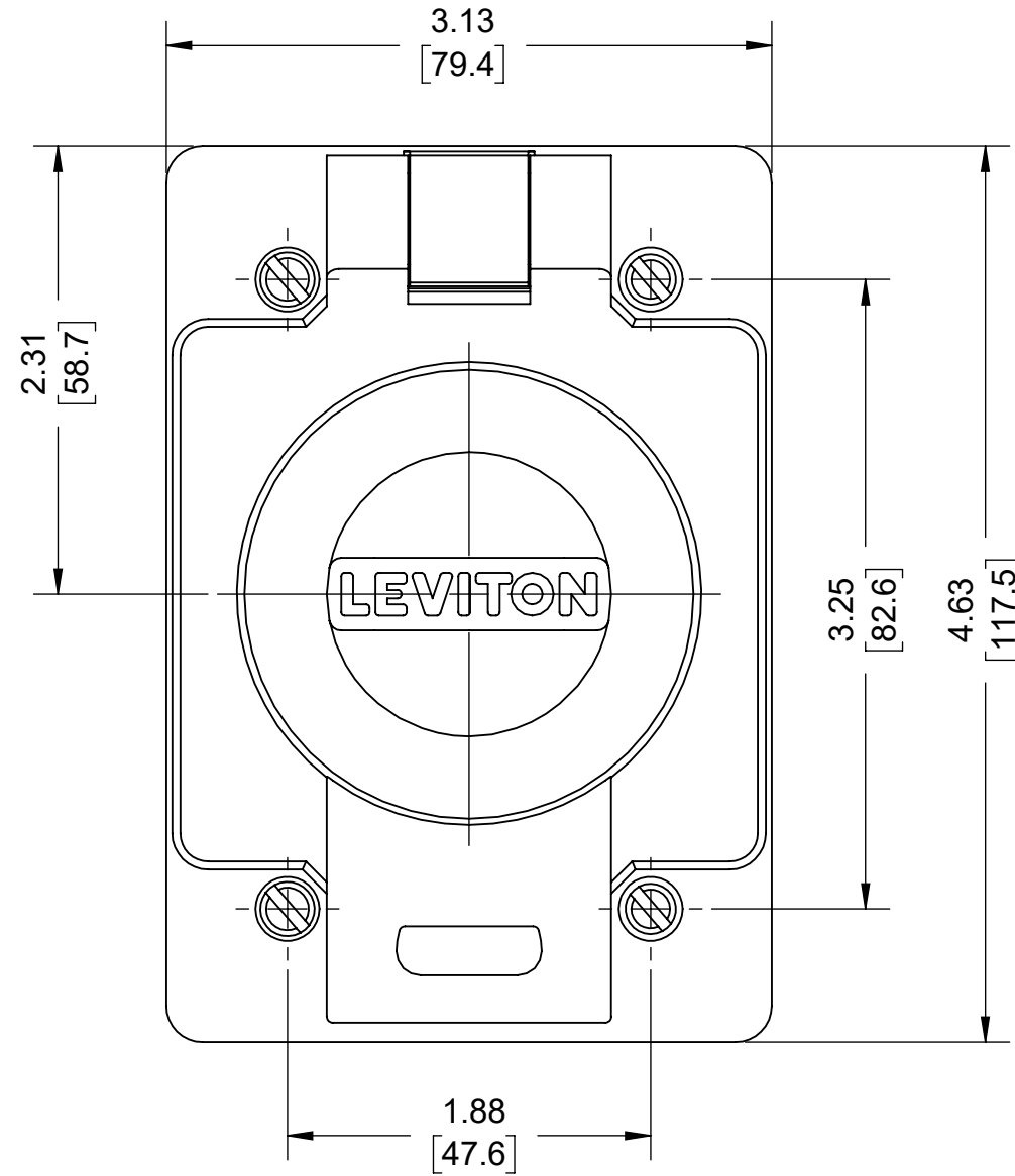
30A 4W WETGUARD FLANGED OUTLET COVER for Cat No 99W74-S
