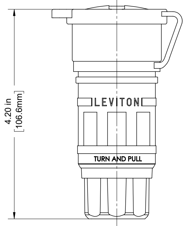
WETGUARD CONNECTOR SHOWN WITH CLOSURE COVER ASSEMBLED
