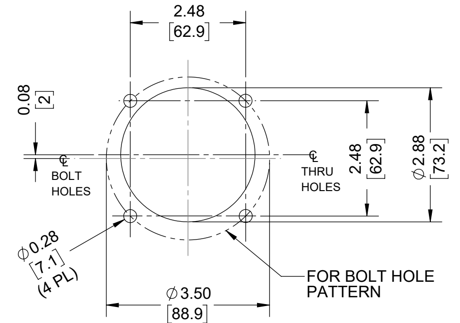
MOUNTING PATTERN FOR 30° MALE & FEMALE PANEL MOUNT RECEPTACLES
