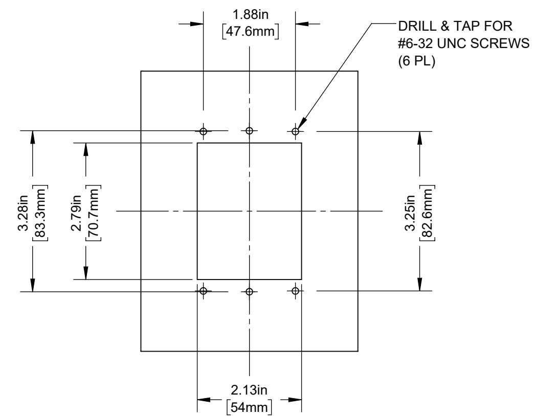
PANEL MOUNT CUT OUT SCALE 1:2
