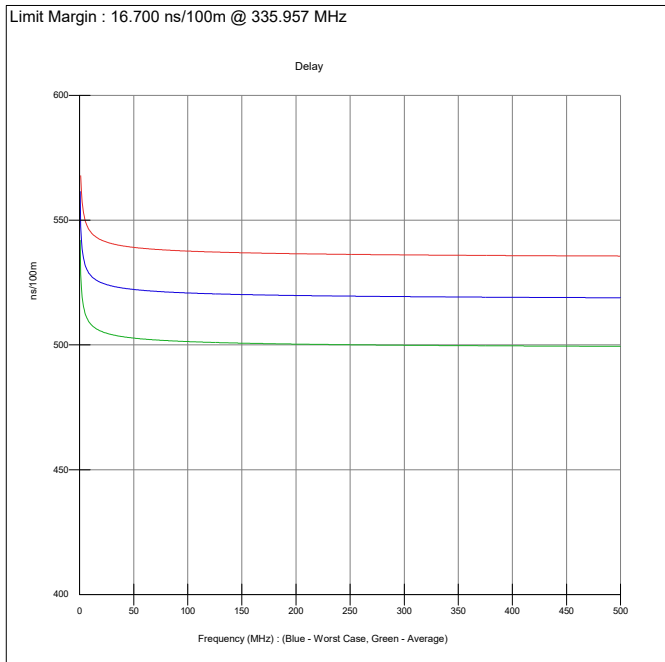
Limit Margin : 16.700 ns/100m @ 335.957 MHz
