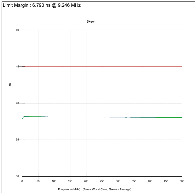
Limit Margin : 6.790 ns @ 9.246 MHz
